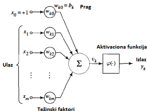
Slika 6.1 Model neurona
